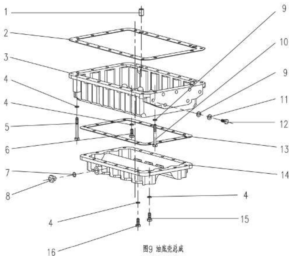
Fig.9 Oil Sump Assembly
